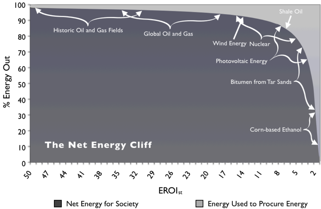
Figure 7: The “Net Energy Cliff” (figure adapted from Lambert and Lambert, in preparation [3] and Murphy et al. 2010 [71]) As EROI approaches 1:1 the ratio of the energy gained (dark gray) to the energy used (light gray) from various energy sources decreases exponentially [71]. High EROI fuels allow a greater proportion of that fuel’s energy to be delivered to society (e.g. a fuel with an EROI of 100:1 (horizontal axis) will deliver 99% of the useful energy (vertical axis) from that fuel to society [71]. Conversely, lower EROI fuel delivers substantially less useful energy to society (e.g. a fuel with an EROI of 2:1 will deliver 50% of the energy from that fuel to society). Therefore, large shifts in high EROI values (e.g. from 100 to 50:1) may have little or no impact on society while small variations in low EROI values (e.g. from 5 to 2.5:1) may have a far greater and potentially more “negative” impact on society [71] (concept courtesy of Euan Mearns).
