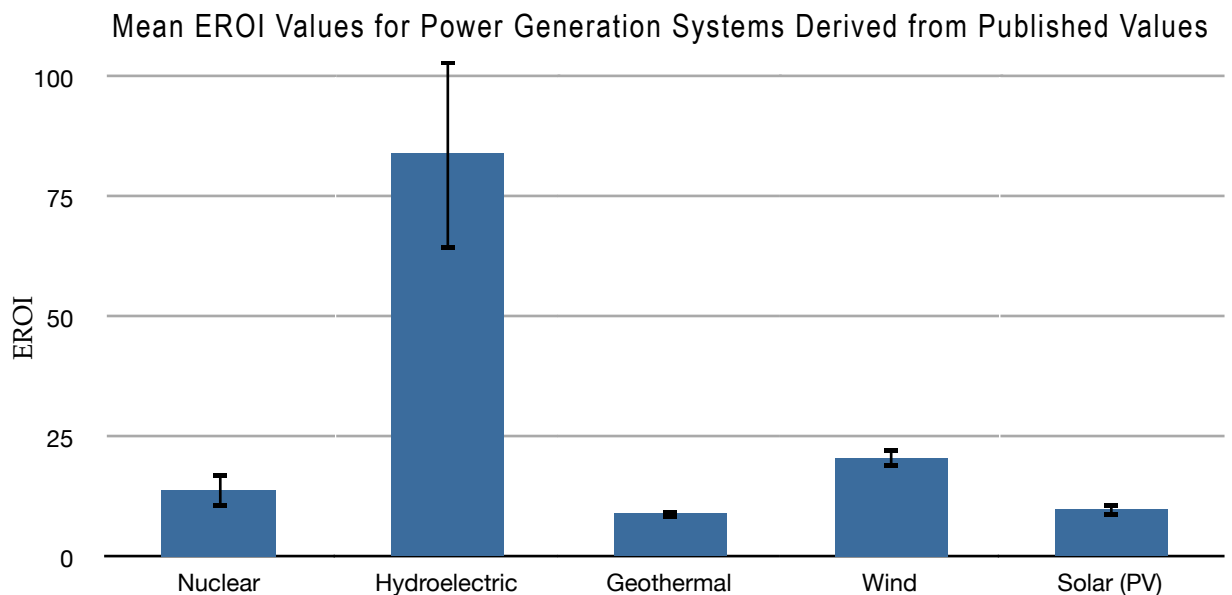
Figure 11: Mean EROI (and standard error) values for known published assessments of power generation systems. Nuclear power has a mean EROI of about 14:1 (n of 33 from 15 publications) [24, 55, 88, 102, 104, 106, 144, 145, 150, 155-160, 197]. Hydroelectric power generation systems have the highest mean EROI value, 84:1 (n of 17 from 12 publications), of electric power generation systems [24, 55, 102, 104, 106, 144-148, 197]. Geothermal electricity production has a mean EROI of approximately 9:1 (n of 30 from 11 publications) [18, 24, 104, 107, 161-163, 197]. Wind power has a mean EROI of about 20:1 (n of 26 from 18 publications) [102, 104, 144, 145, 147, 148, 164-171, 197]. Solar (photovoltaic) power generation has a mean EROI of roughly 10:1 (n of 79 from 45 publications) [24, 55, 104, 106, 144, 145, 147, 148, 153, 154, 167, 168, 150, 170, 172-197].
